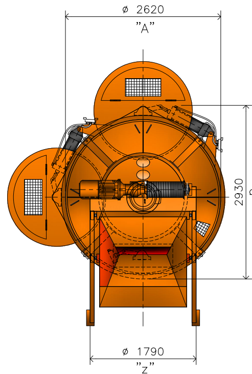
Technical sheet used mixer Concretelle 1500/1000 with skip-hoist:
